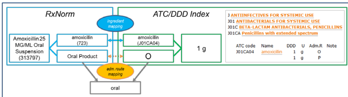
Figure 6. Mapping between RxNorm and ATC through both the ingredient and the route of administration
