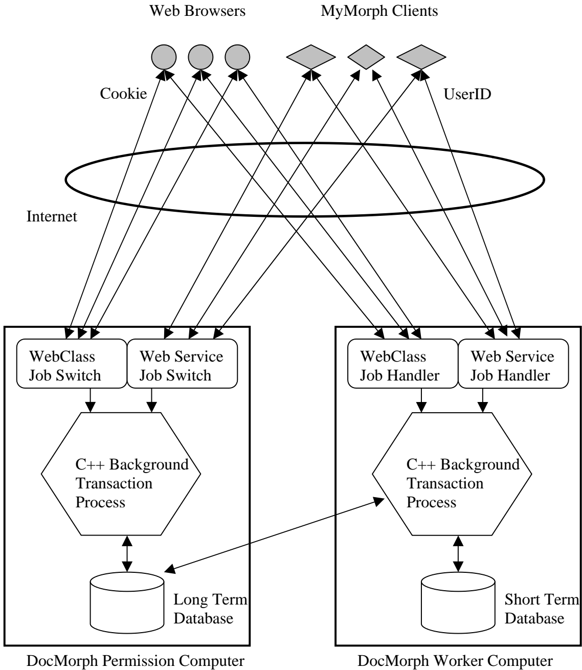
Figure 2. DocMorph System Architecture
